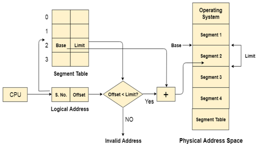
Fig. 2 Translation of Logical address into physical address by segment table
